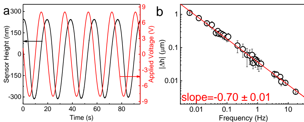
Figure 2: (a) Electromechanical response at the center of the actuator measured with a scanning probe microscope (SPM) in semi-contact mode. Both the probe and the top contact are at ground potential. The figure shows sensor height as a function of time with 8V, 50mHz applied voltage. Baseline was subtracted in order to compensate for thermal drift. (b) Log-log plot of the amplitude of ECM response vs bias frequency at 8V. Six samples were measured and their response averaged. Response amplitude is found to scale inversely with frequency ( f ) between 5mHz and 20Hz according to |\Delta h| \propto f^{-0.7} with R_{adj}^2 = 0.99807 .
