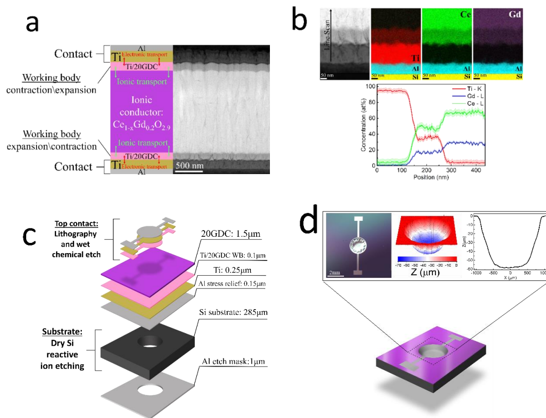
Figure 1: (a) Scheme of the ECM actuator showing its basic elements and practical realization. TEM micrograph of a 70-100 nm thick cross section slice of the multilayer stack deposited on a Si substrate. (See section 4 for fabrication details). (b) High resolution (1nm spot size) TEM energy dispersive spectroscopy (EDS) elemental mapping, providing elemental composition of the Si, Al, Ti, WB and 20GDC solid electrolyte layers. (c) Schematic representation of the sputtered layer stack. The structure is transformed into a 2mm diameter, tethered membrane by means of dry Si etching, lithographic patterning and wet chemical metal etch. (d) Image of the membrane buckling pattern and depth profile as measured by an optical profiler (see section 2 in supporting information for details).
