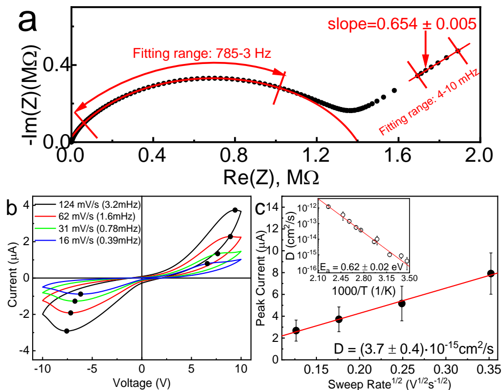
Figure 4: (a) Nyquist plot of ECM actuator impedance at 354 mV excitation voltage, 1MHz-4mHz at room temperature. The high frequency arc can be fit to a depressed circle (radius R_0 ), centered at (x_0, y_0) in the complex plane: -im(Z) = y_0 + [R_0 - (Re(Z) - x_0)^2]^n (Equation. (3)) with y_0 = 226(\pm 1.4\%) k \Omega , x_0 = 693(\pm 0.04\%) k \Omega , R_0 = 771(\pm 0.2\%) k \Omega , n = 0.488(\pm 0.03\%) , R_{adj}^2 = 0.99999 . The slope of the low frequency constant phase element is: 0.654 \pm 0.005 , R_{adj}^2 = 0.9997 . (b) Room temperature cyclic voltammograms with sweep rates 16-124 mV/s, bottom contact at ground potential. Current peaks ( I_p ), indicating a reversible, diffusion limited, charge transfer process, were identified by double differentiation of the voltammogram and are indicated. (c) Peak current as a function of the square root of the sweep rate, averaged over positive and negative applied voltage, for 10 samples. The slope, determined by linear regression, is used to extract the diffusion coefficient according to the Randles Sevcik equation (Equation. (4)). Inset: Arrhenius plot of the ion diffusion coefficient between 16-170°C averaged for 7 samples. See Figure S5, section 5 in supplementary information for temperature dependent cyclic voltammograms. Activation energy ( E_a ) for ion diffusion, 0.62 \pm 0.02 eV.
