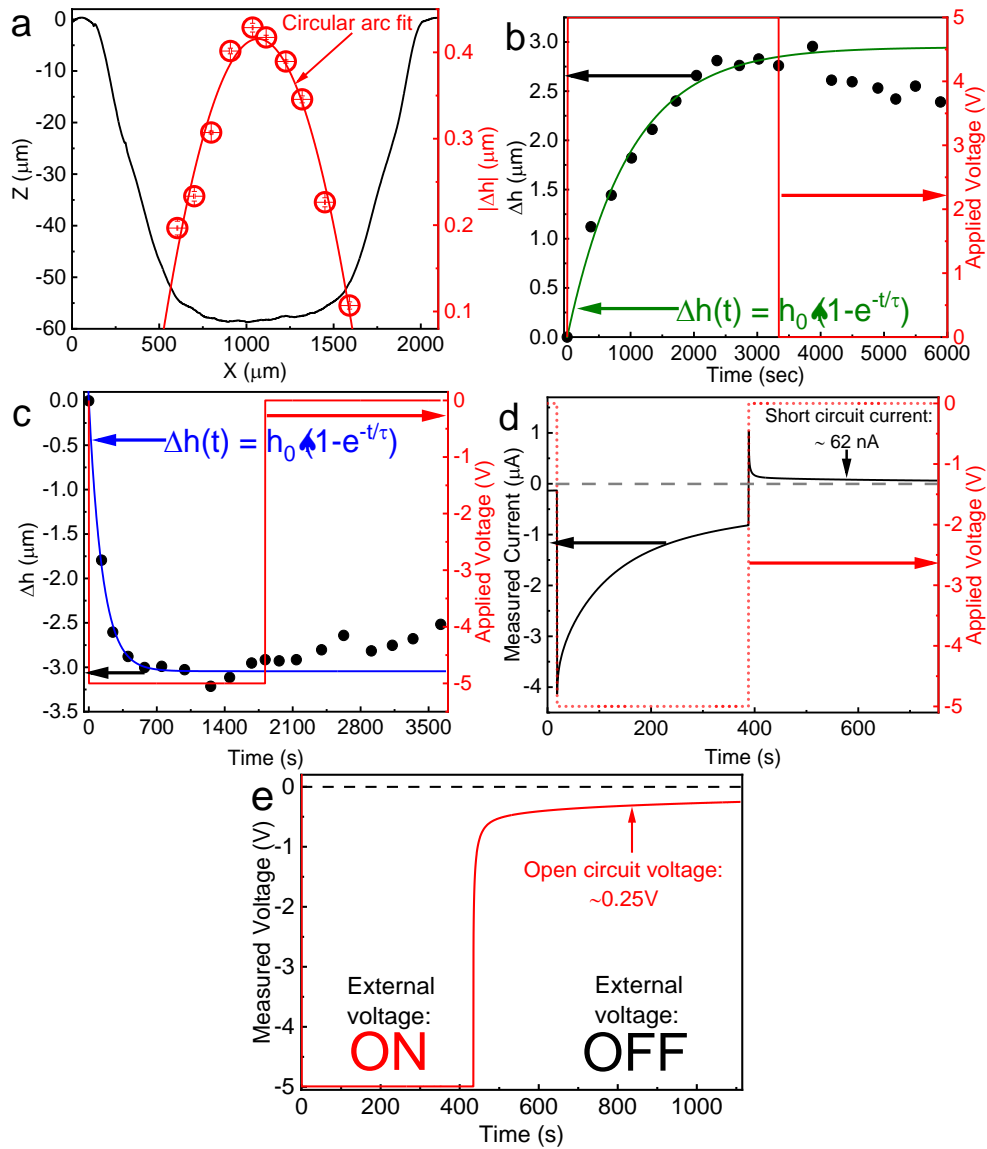
Figure 3: (a) (o) The lateral distribution of the amplitude of the electromechanical response ( |\Delta h| ) of the central 1mm diameter region of the membrane to 8V 50mHz as measured with the scanning probe microscope. The microscope tip and top contact were at ground potential. The distribution may be fit by a circular arc with radius 435(\pm 7\%) mm. (—) The shape of the buckled, tethered membrane as determined by the optical profiler in the absence of applied voltage. (b,c) Vertical displacement ( \Delta h ) at the center of the membrane with constant \pm 5 V applied bias, as measured with an optical profiler, increased with time according to \Delta h(t) = h_0 \cdot (1 - e^{-t/\tau}) giving characteristic response time of \tau_{+5V} = 980 \pm 75 s, h_{0,+5V} = 2.95 \pm 0.08 \mu\text{m} and \tau_{-5V} = 139 \pm 9 s, and h_{0,-5V} = 3.04 \pm 0.03 \mu\text{m} . Only weak relaxation was observed during more than 2500 s following bias removal. (d) Membrane charge/discharge cycle showing short circuit current of \sim 62 nA when -5 V DC is removed after 380 sec. (e) Membrane charge/discharge cycle showing open circuit voltage of \sim -0.25 V when -5 V DC is removed after 440 sec. For measurements performed in b-e, the bottom contact was at ground potential.
